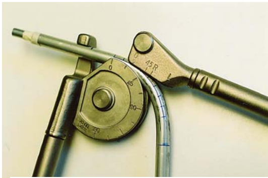
3. Tubing bender tool forms the nose gear strut. Strut can also be purchased.
