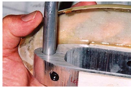
4. Nose gear strut fits into nose gear fork, squeezed by socket head bolt. Easily removeable and adjustable.
