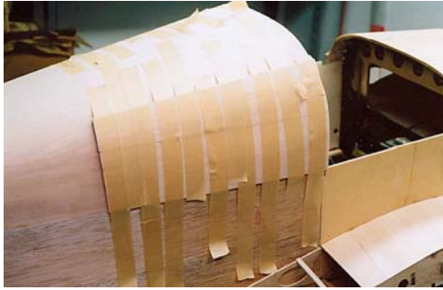
25. Two layers of balsa sheet are formed over rear window area. Held with masking tape.
