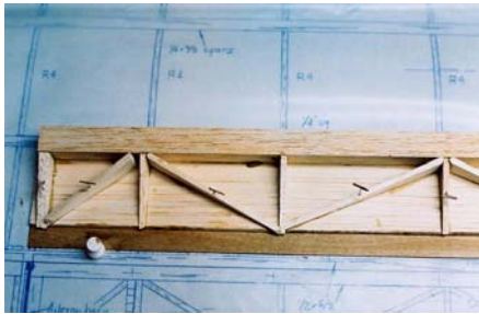
11. Ailerons and flaps are assembled on a flat surface. Ply strip forms sharp trailing edge.
