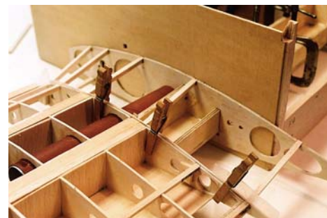
16. Gluing root rib and wing tube sockets in place. Tips elevated per diagram on plans. Verify equal incidence angles of both wings with incidence meter before glue sets. Wing is only partially sheeted at this point.
