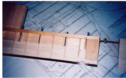
20. Elevator halves joined and hinged before bottom sheeting is completed.
