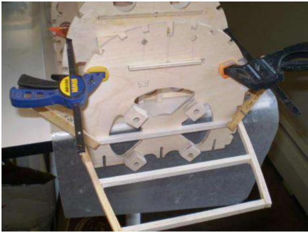
With crutch hanging over the edge, glue the firewall F3 in place. Before glue sets, trust but verify that the LiPo batteries will fit.
