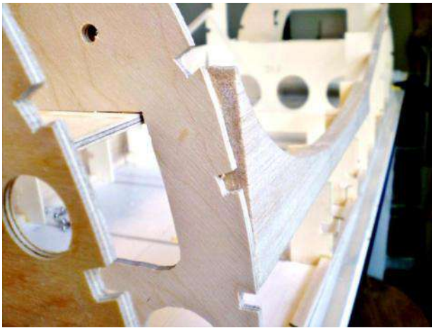
Plane the wing saddle to blend into F7.
