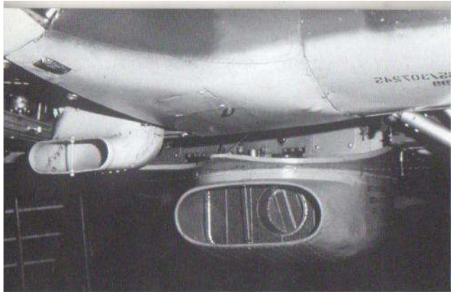
The radiator bath on all Hurricanes is located just to the rear of the landing gear bay. A stencil on the port side states the recommended coolant mixture is 70% water and 30% glycol. This is the later, and most common radiator with the circular oil cooler. The small scoop in the foreground is the carburetor air-intake.
