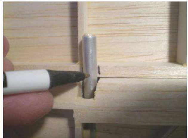
Add a ply patch to the lower spar where the bolts will be. Position the elevators over the stab's trailing edge spar. Mark the locations of the hinge extensions.
