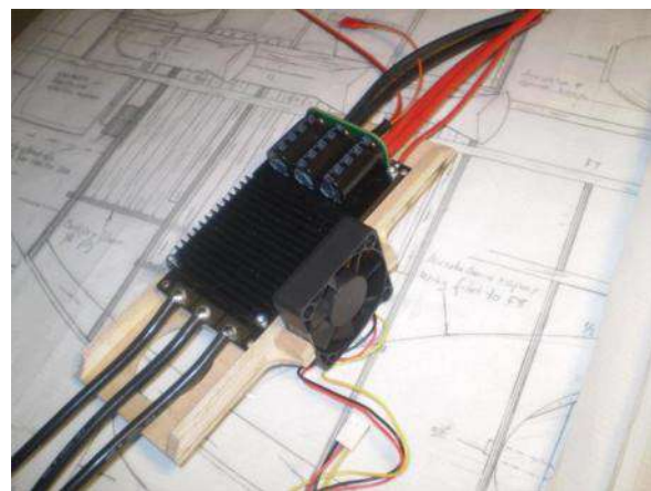
ESC in its holder, ready to install in fuselage.
