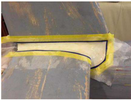
Light weight glass cloth is applied with epoxy resin. After curing, the excess is trimmed away with a razor blade.
